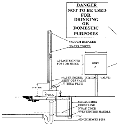
Figure II – Flushing Device
